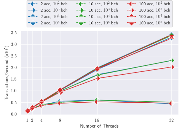
Fig. 6. Throughput of SPEEDEX on batches of payment transactions with varying thread counts (average of 100 trials).
